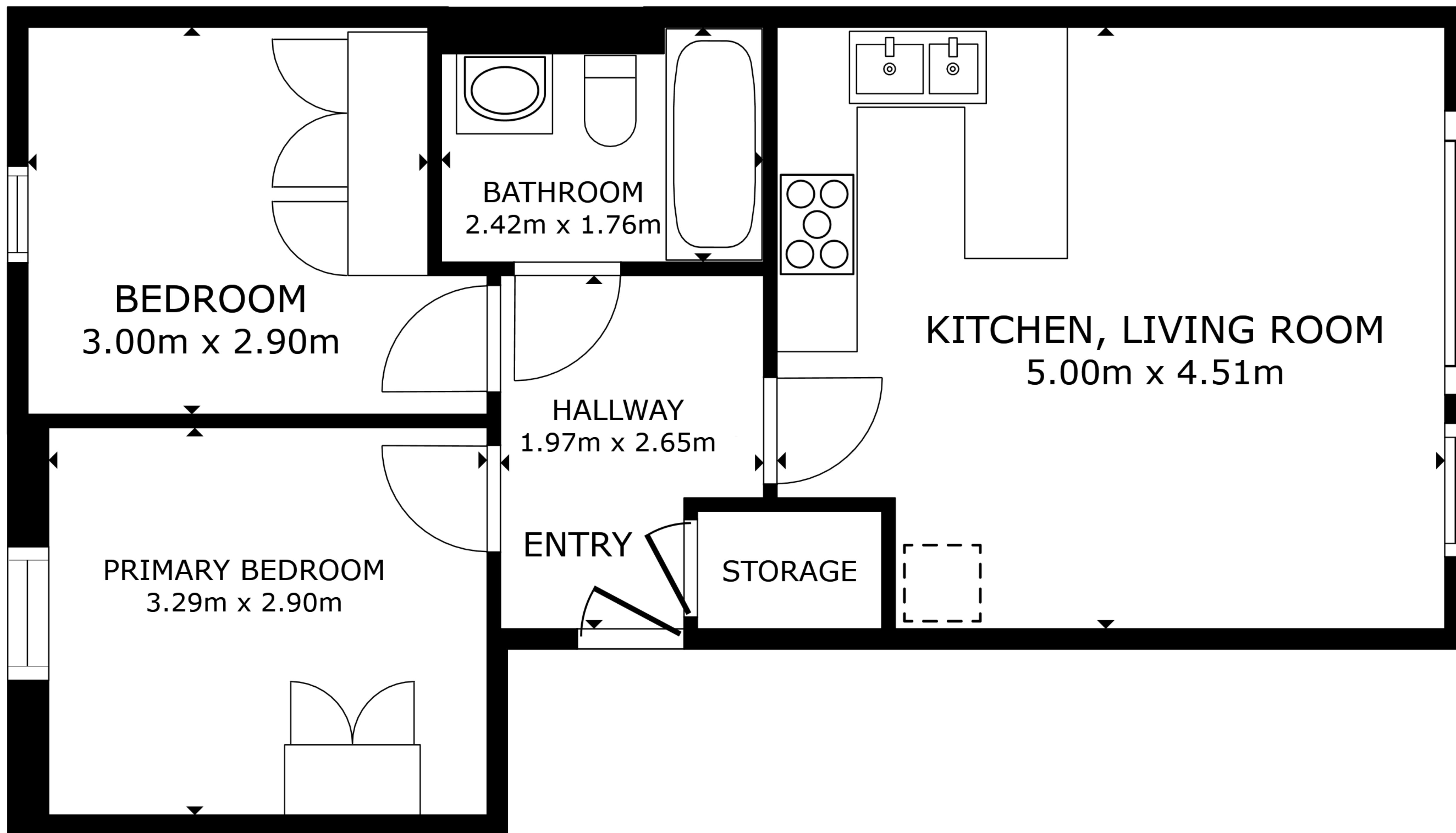
FLOOR PLAN
