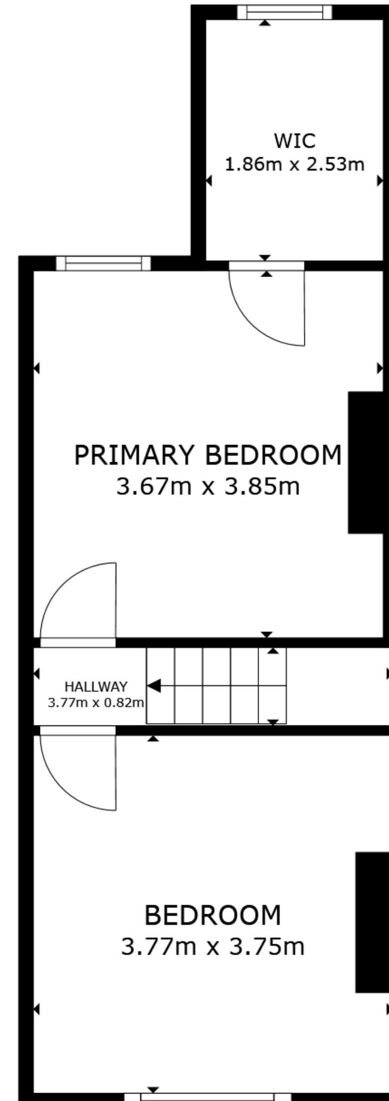
FLOOR 2
