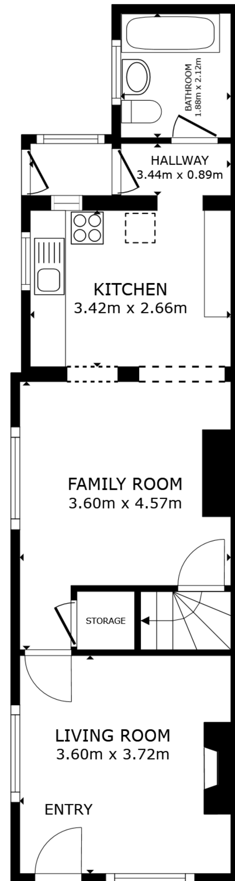
FLOOR 1
