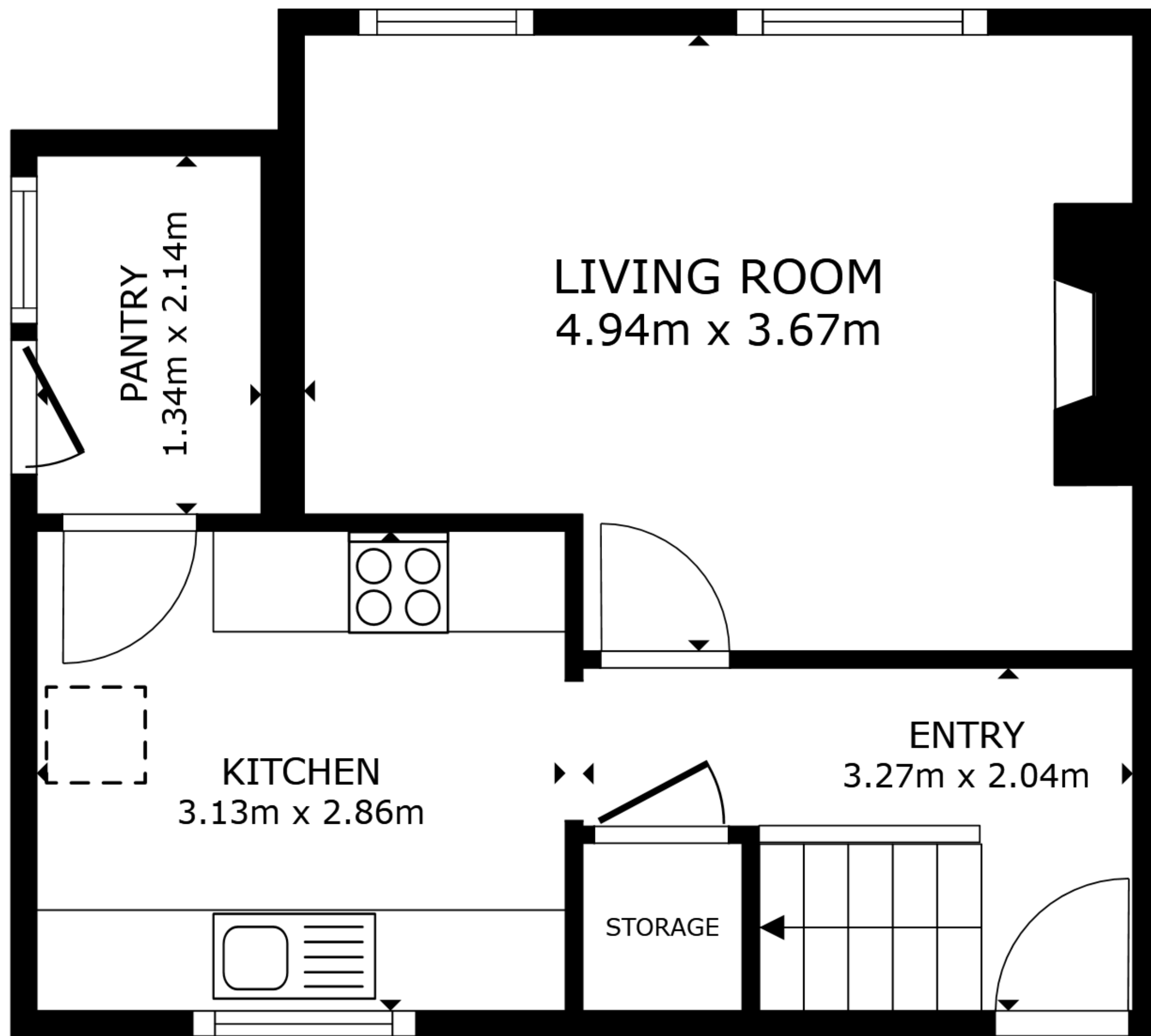
FLOOR 1
