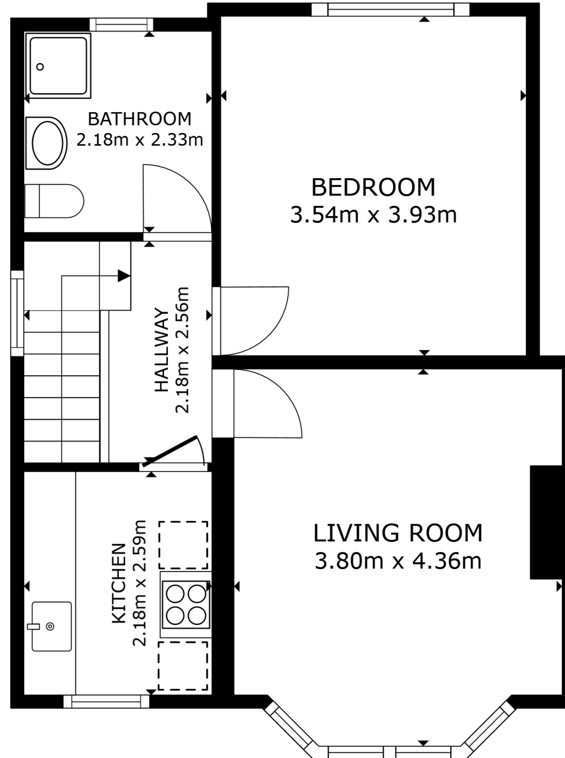
FLOOR 2
