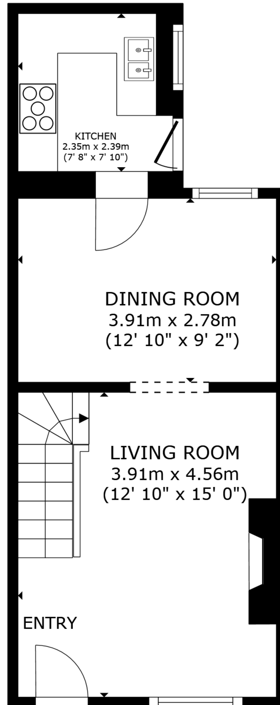
FLOOR 1
