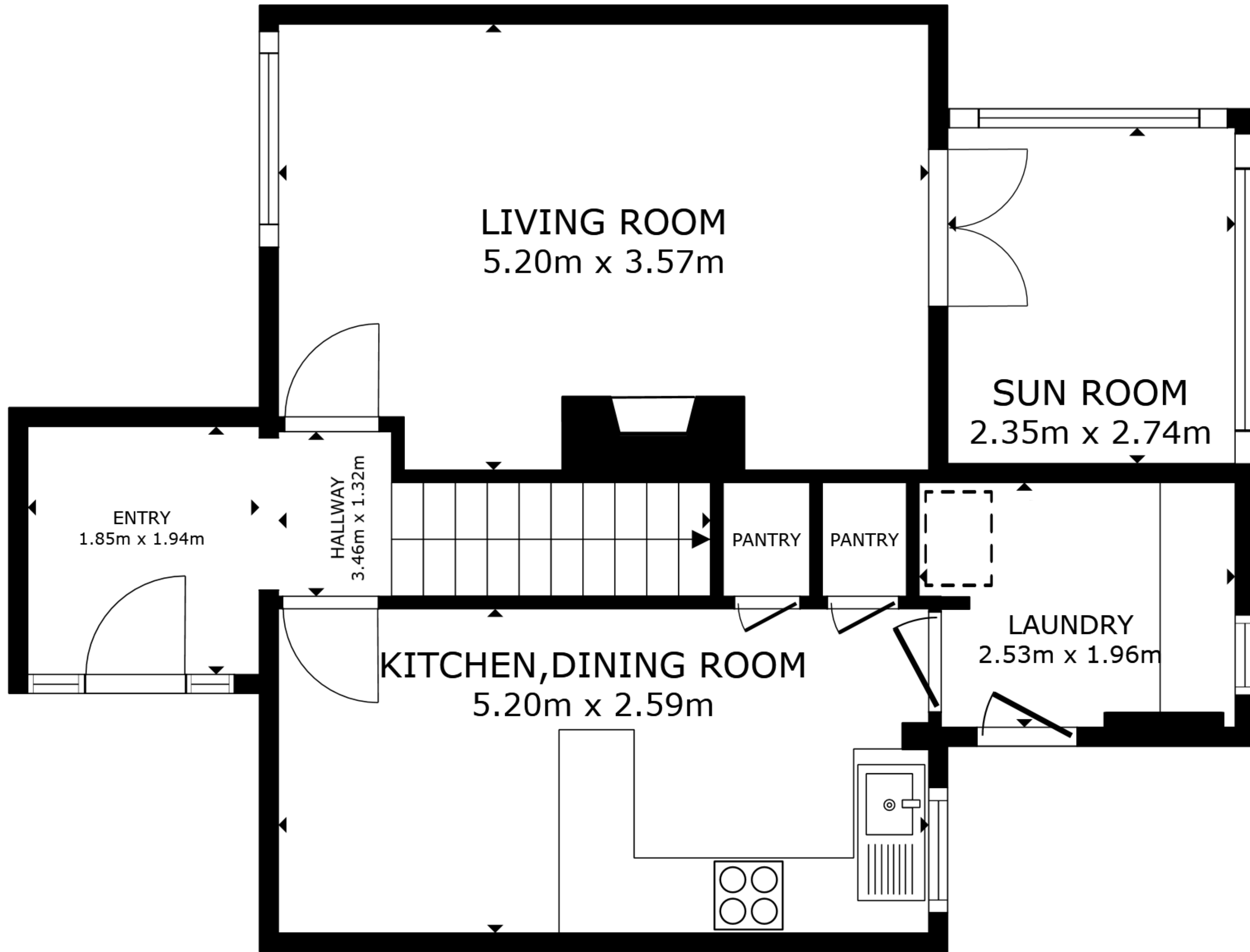
FLOOR 1
