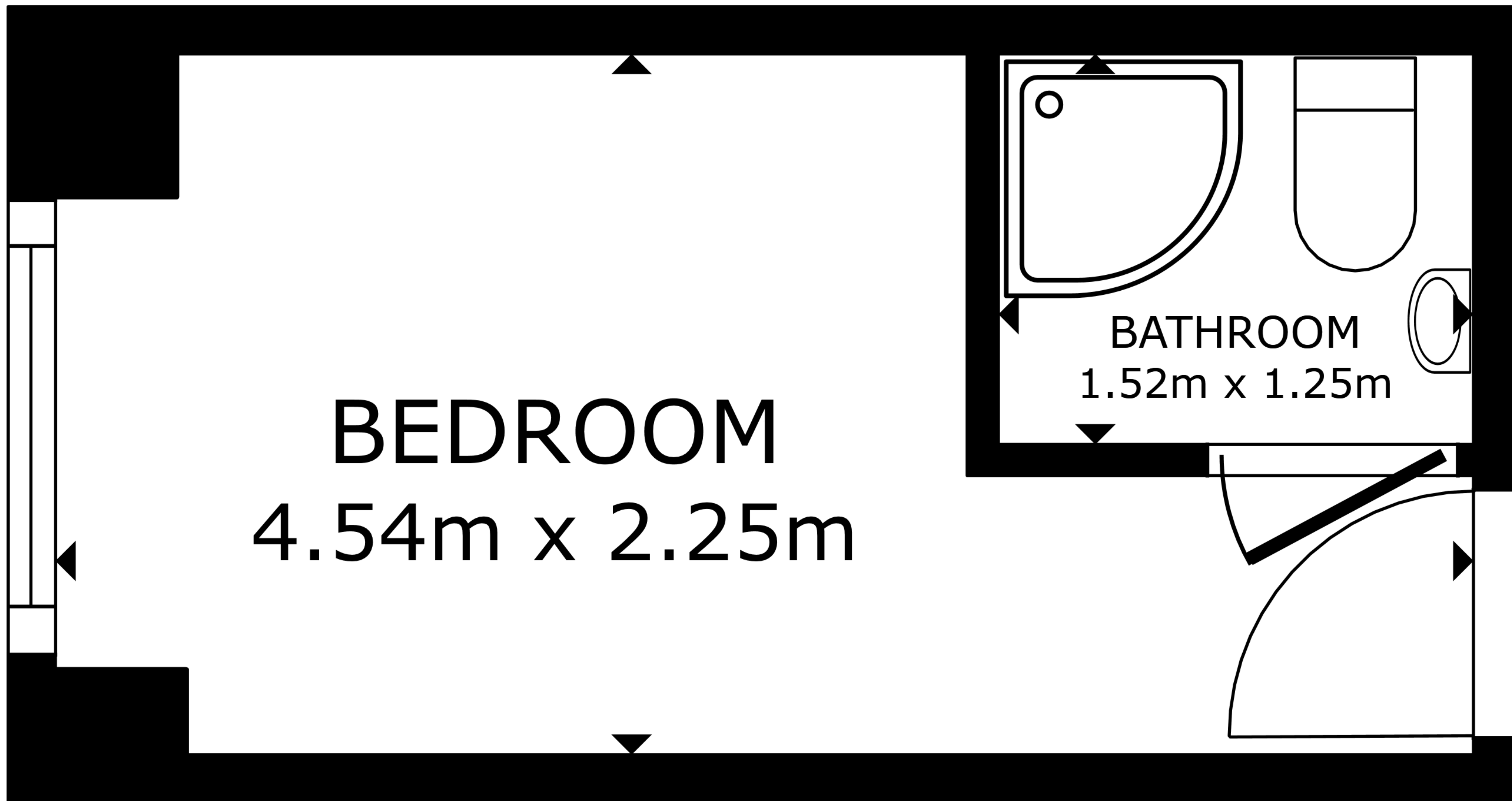
FLOOR PLAN
