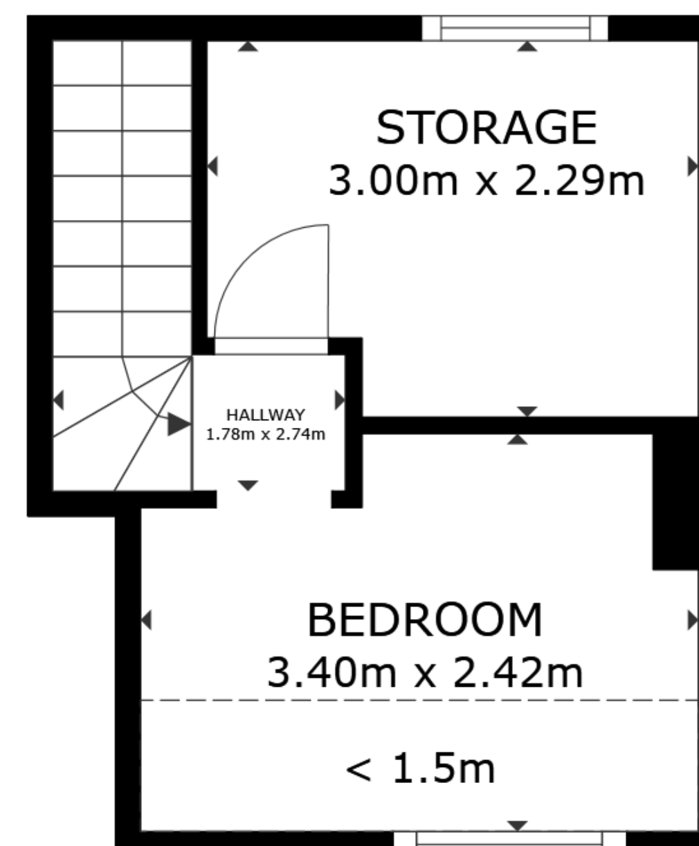
FLOOR 2
