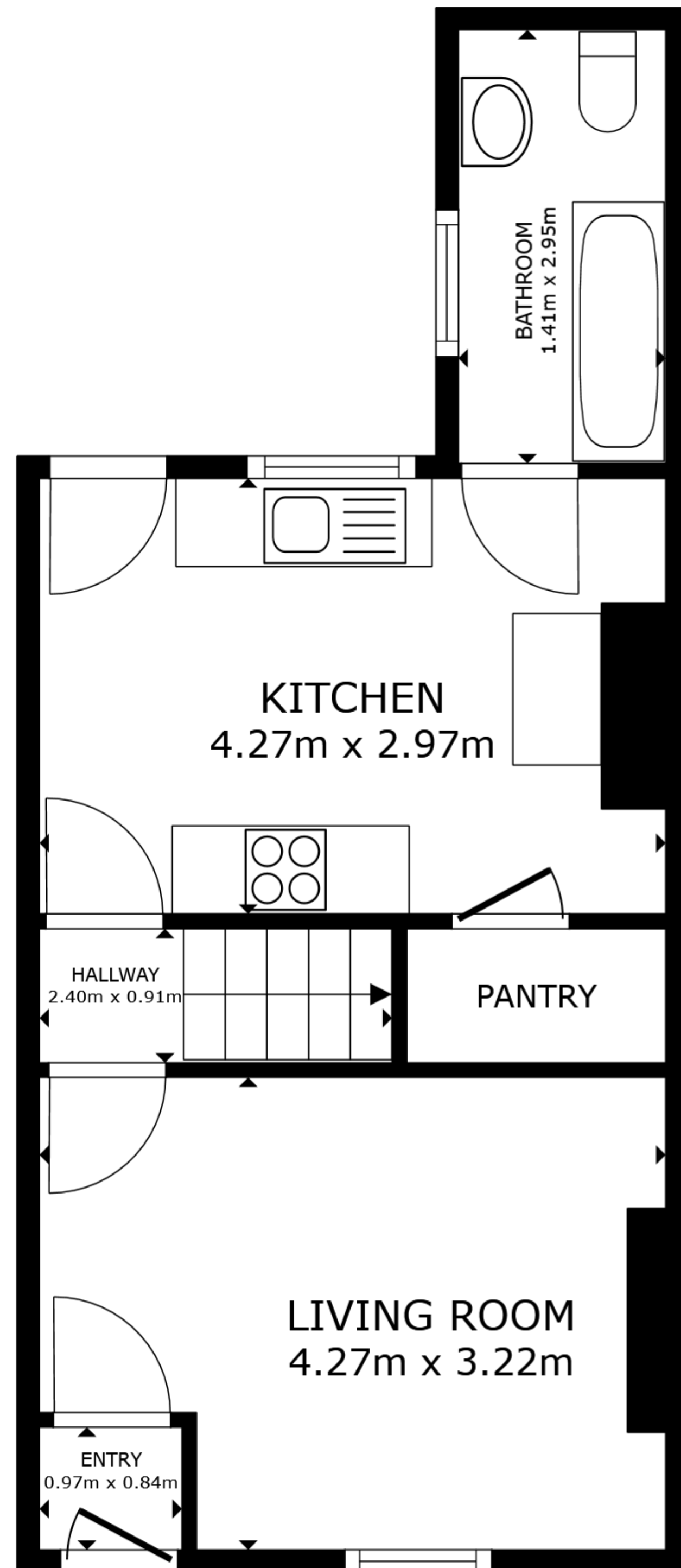
FLOOR 1
