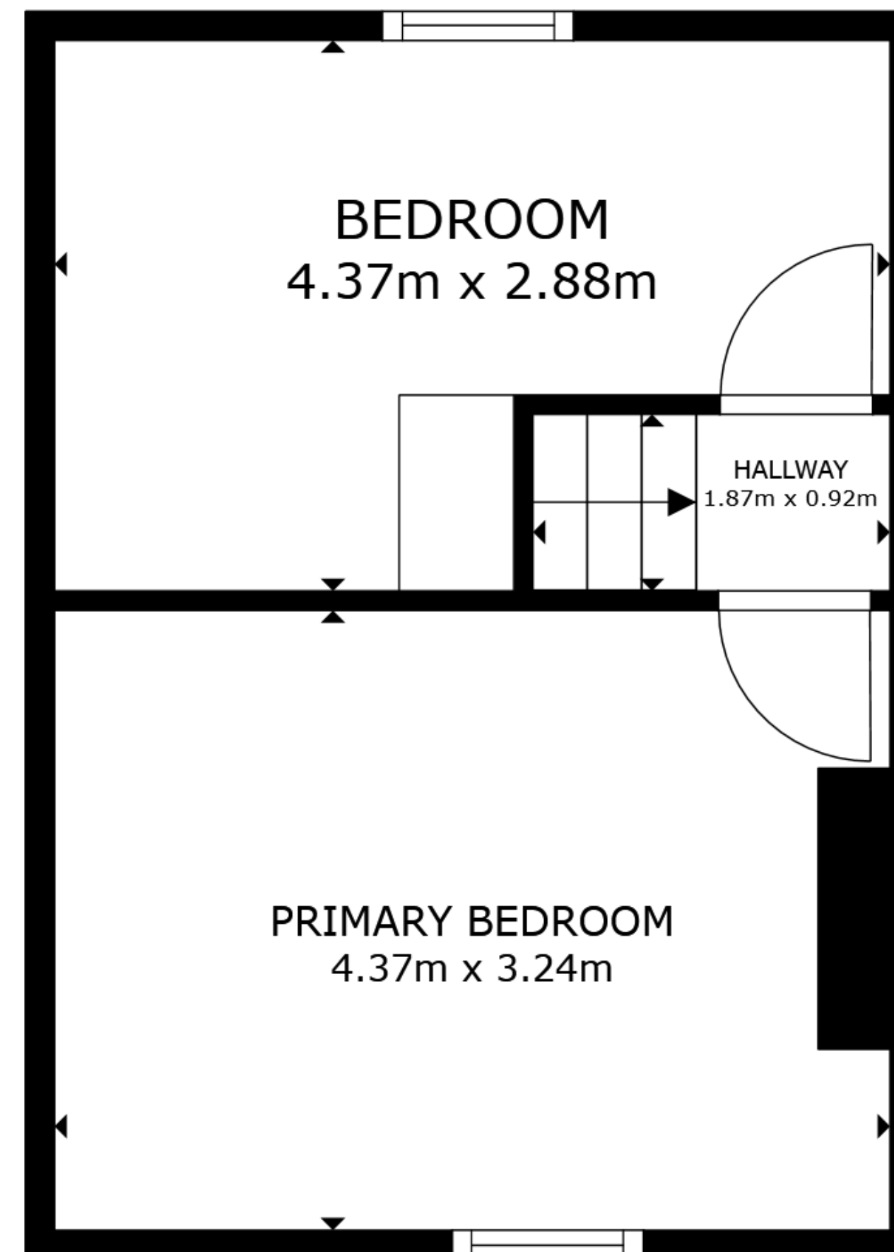
FLOOR 2
