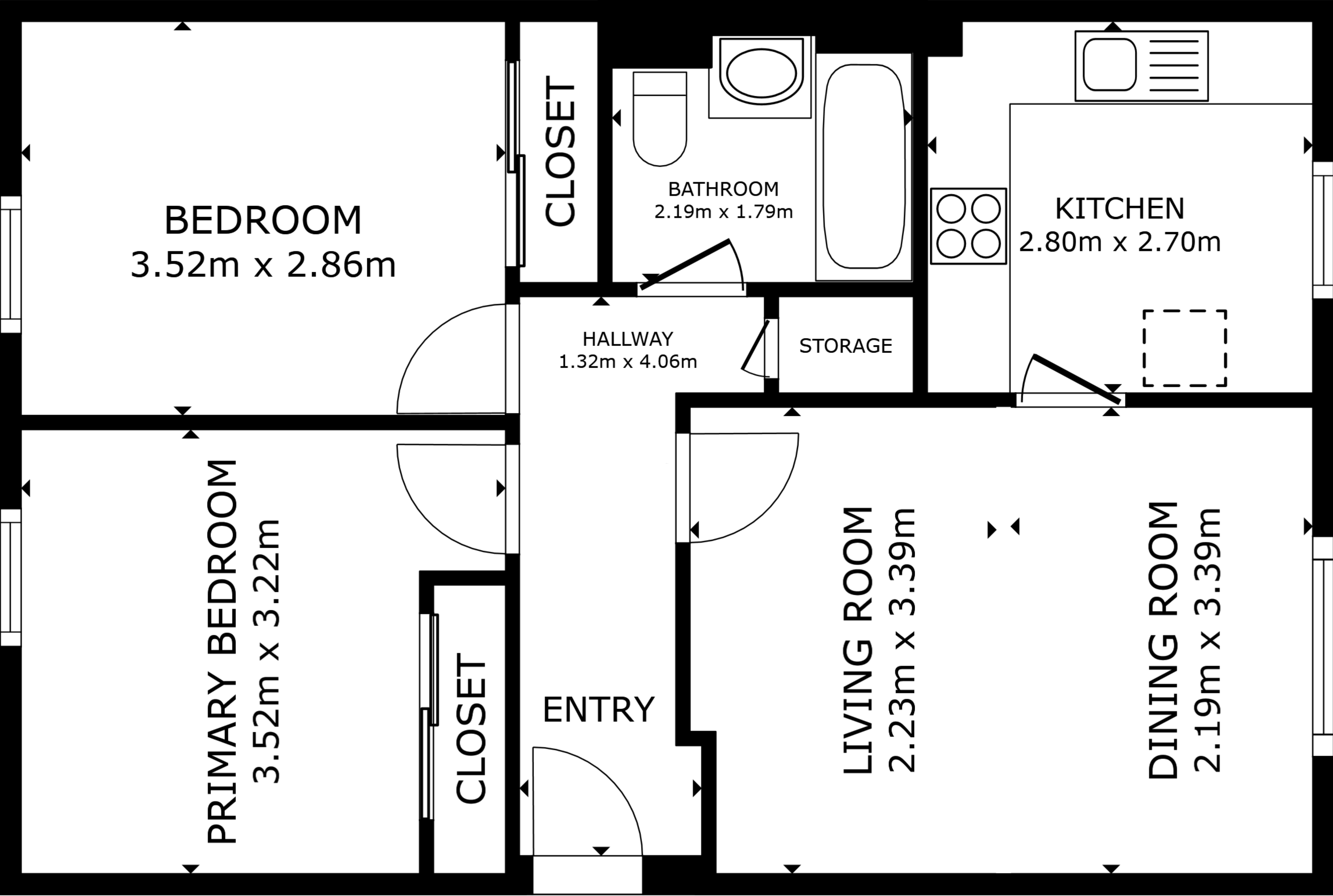
FLOOR PLAN
