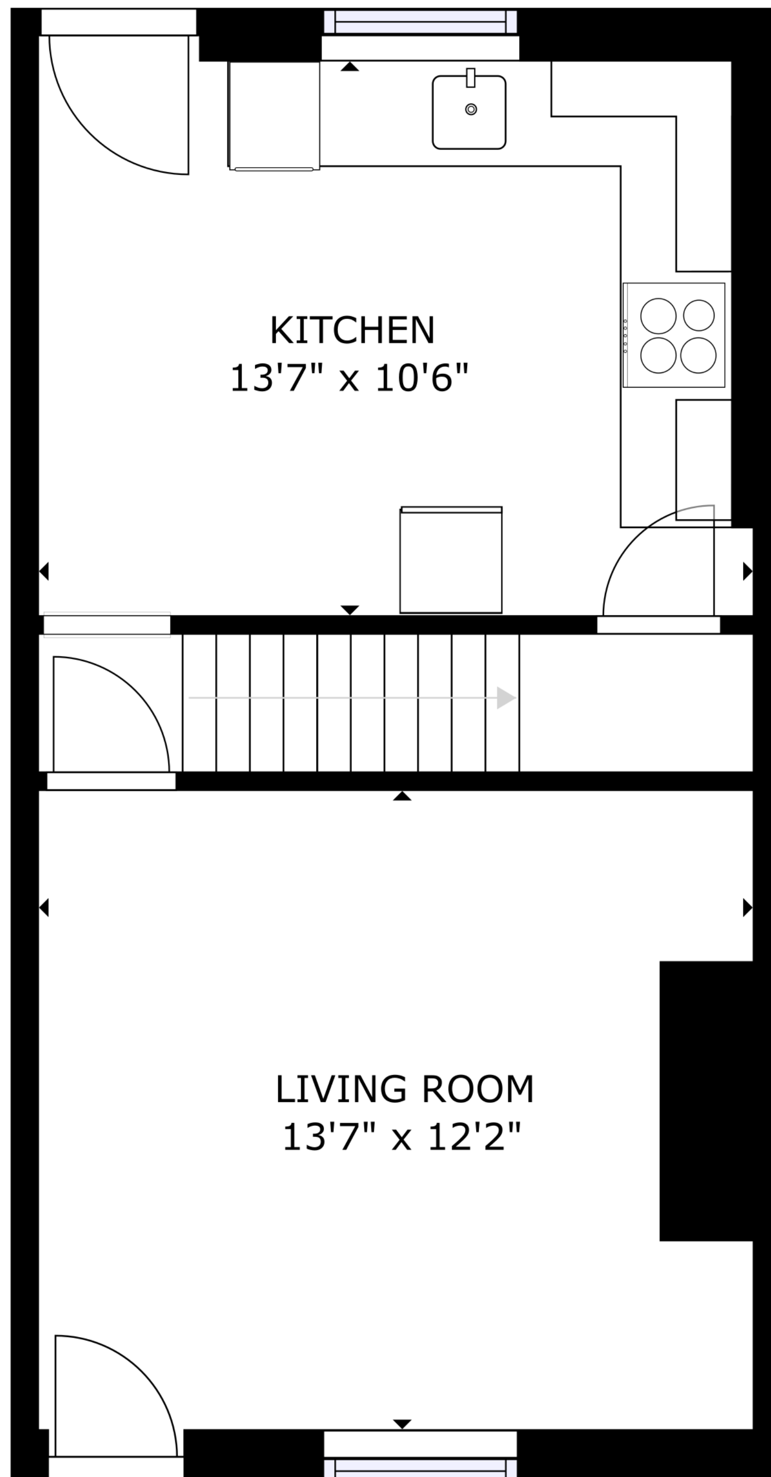
FLOOR 1
