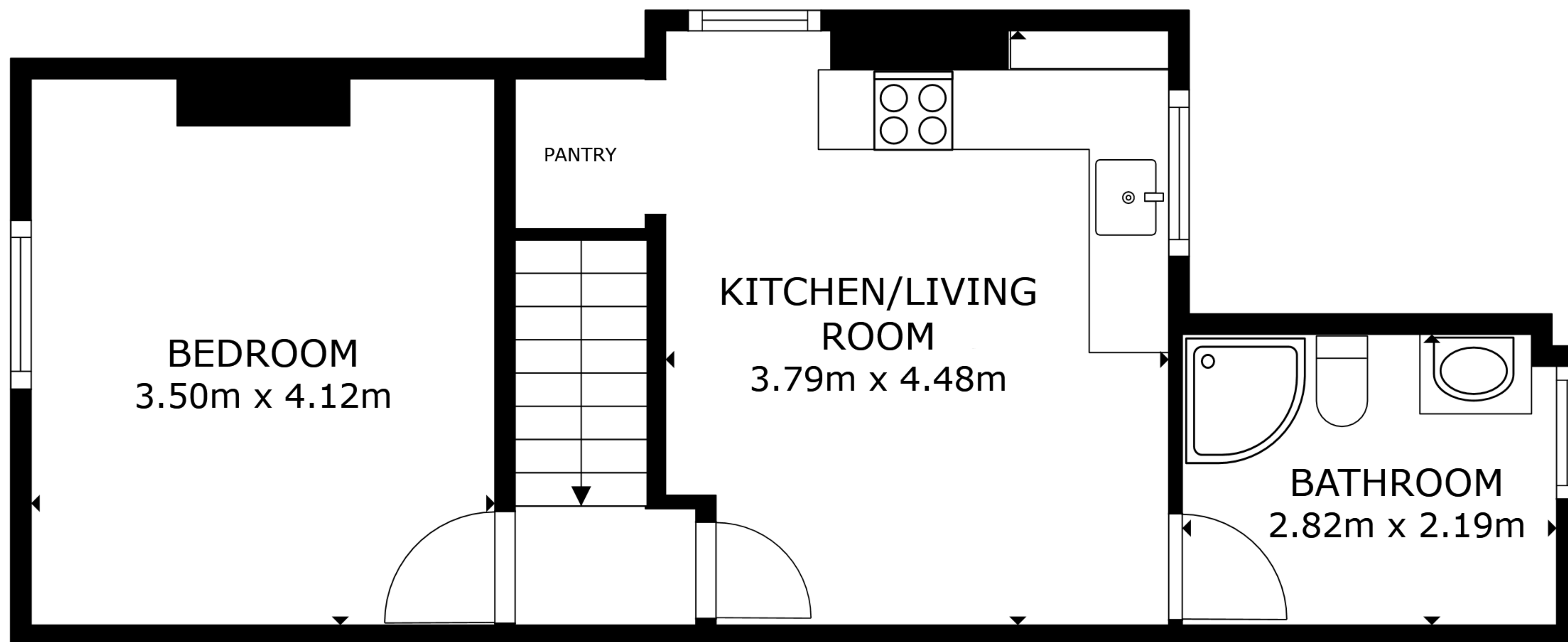
FLOOR PLAN
