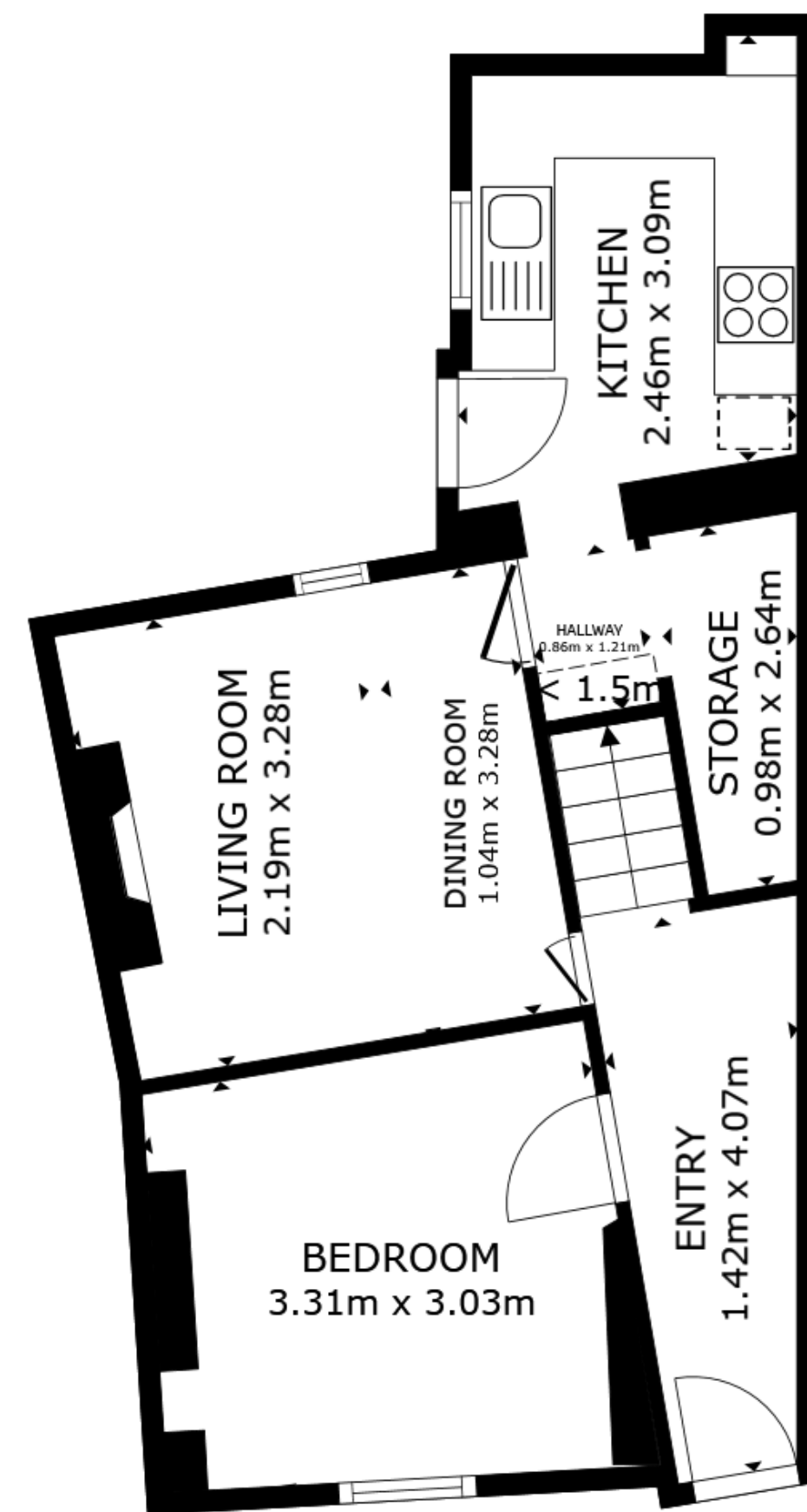
FLOOR 1
