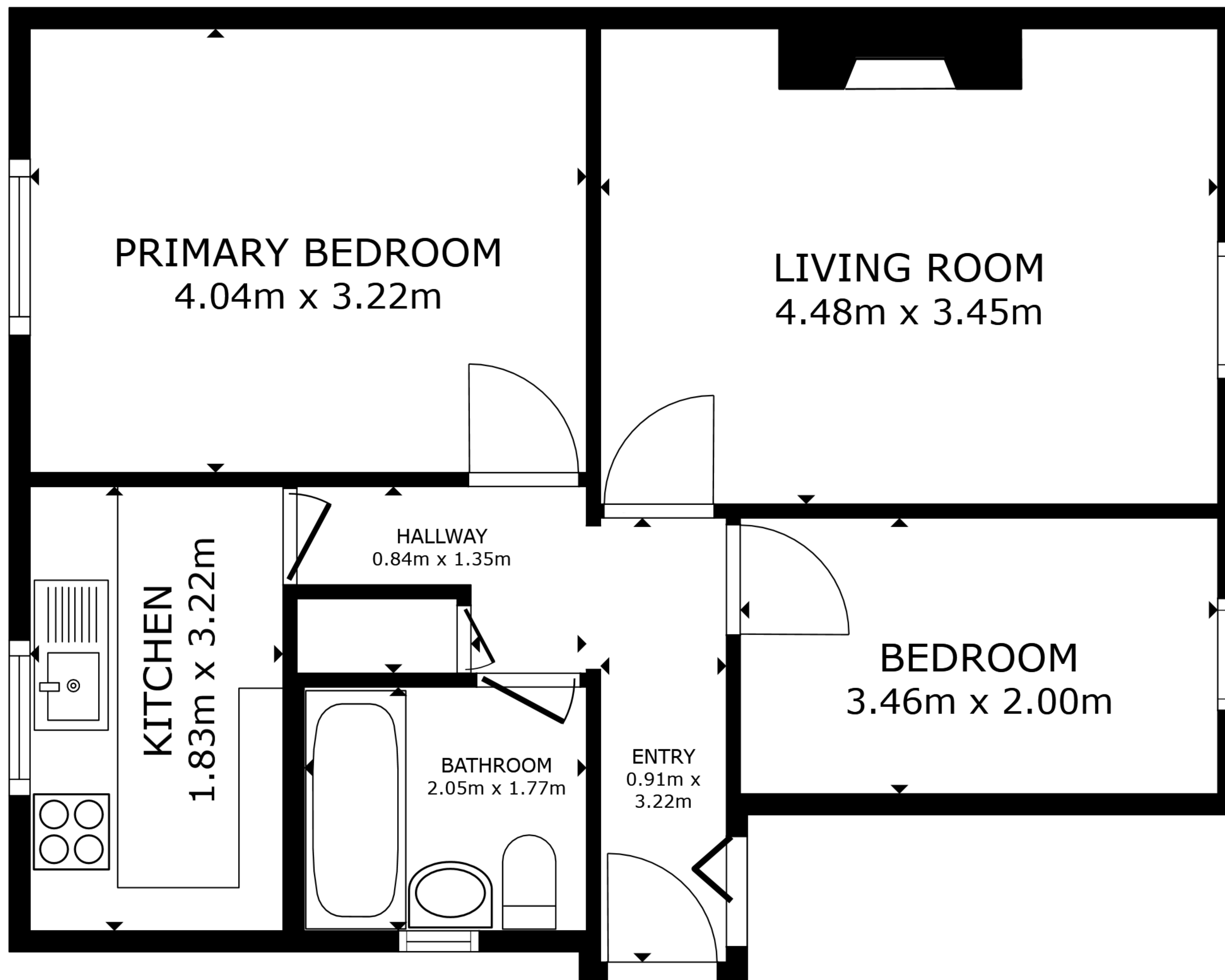
FLOOR PLAN
