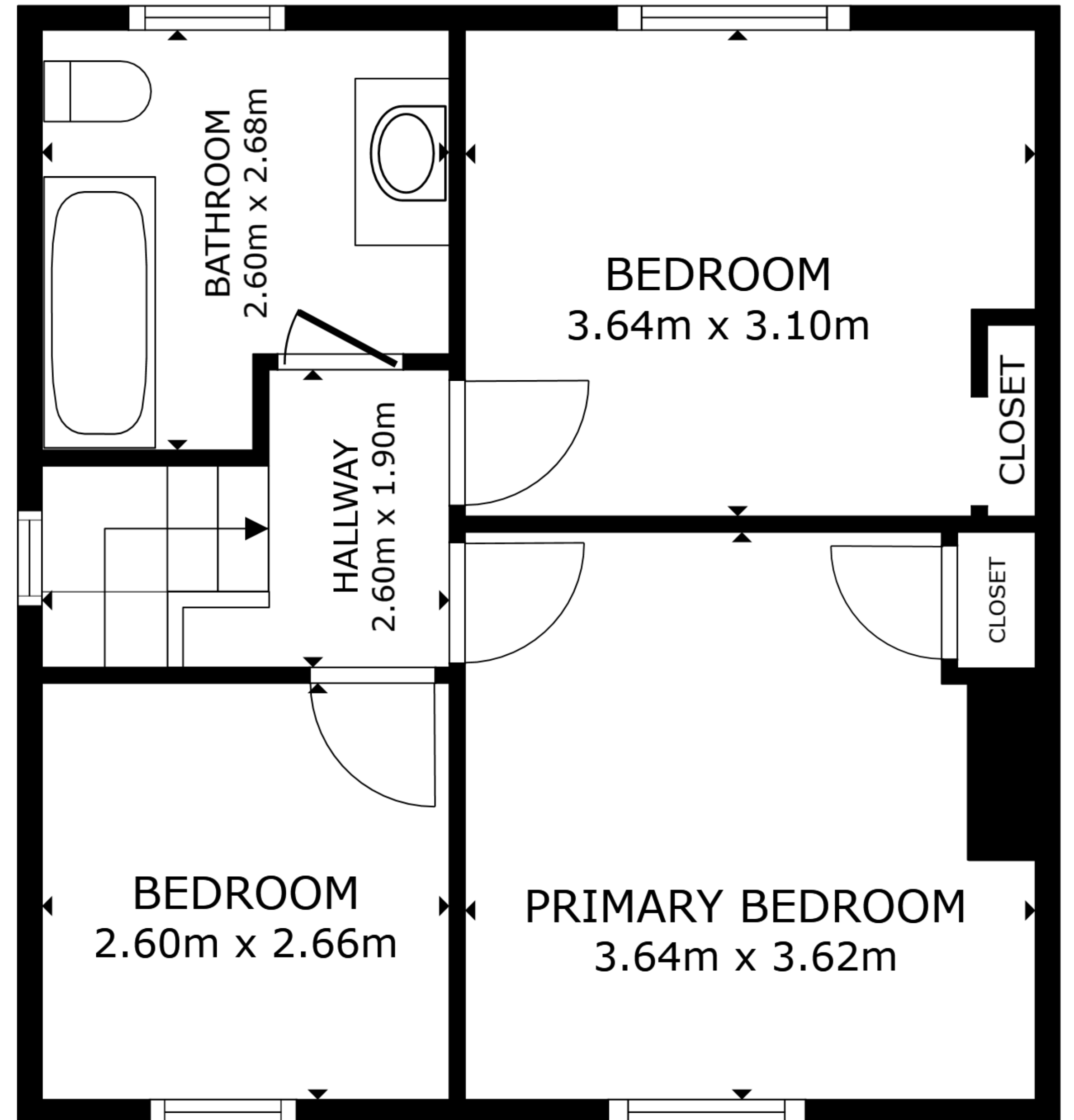
FLOOR 2
