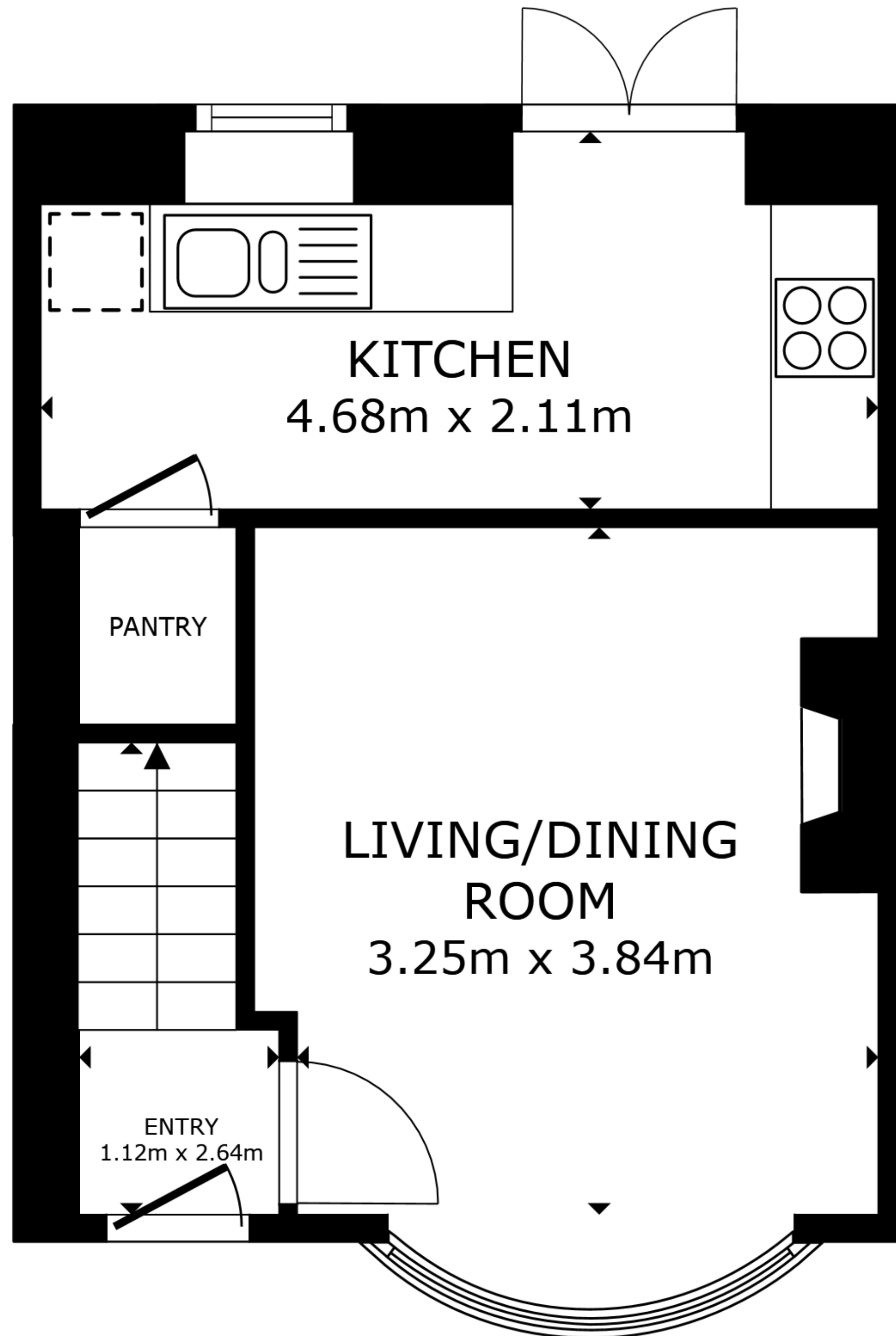
FLOOR 1
