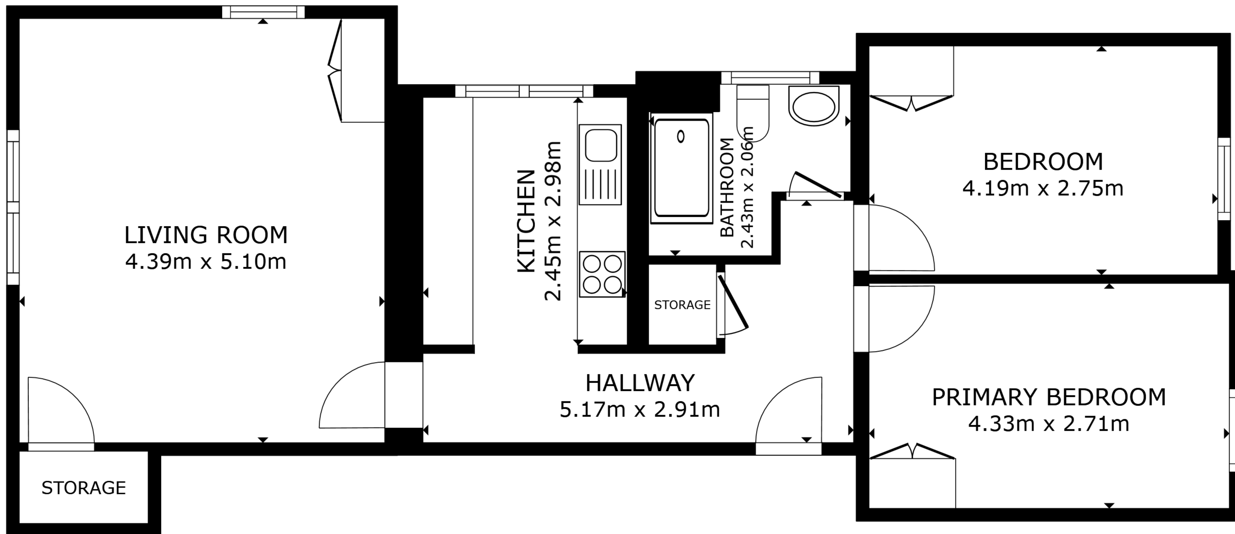
FLOOR PLAN
