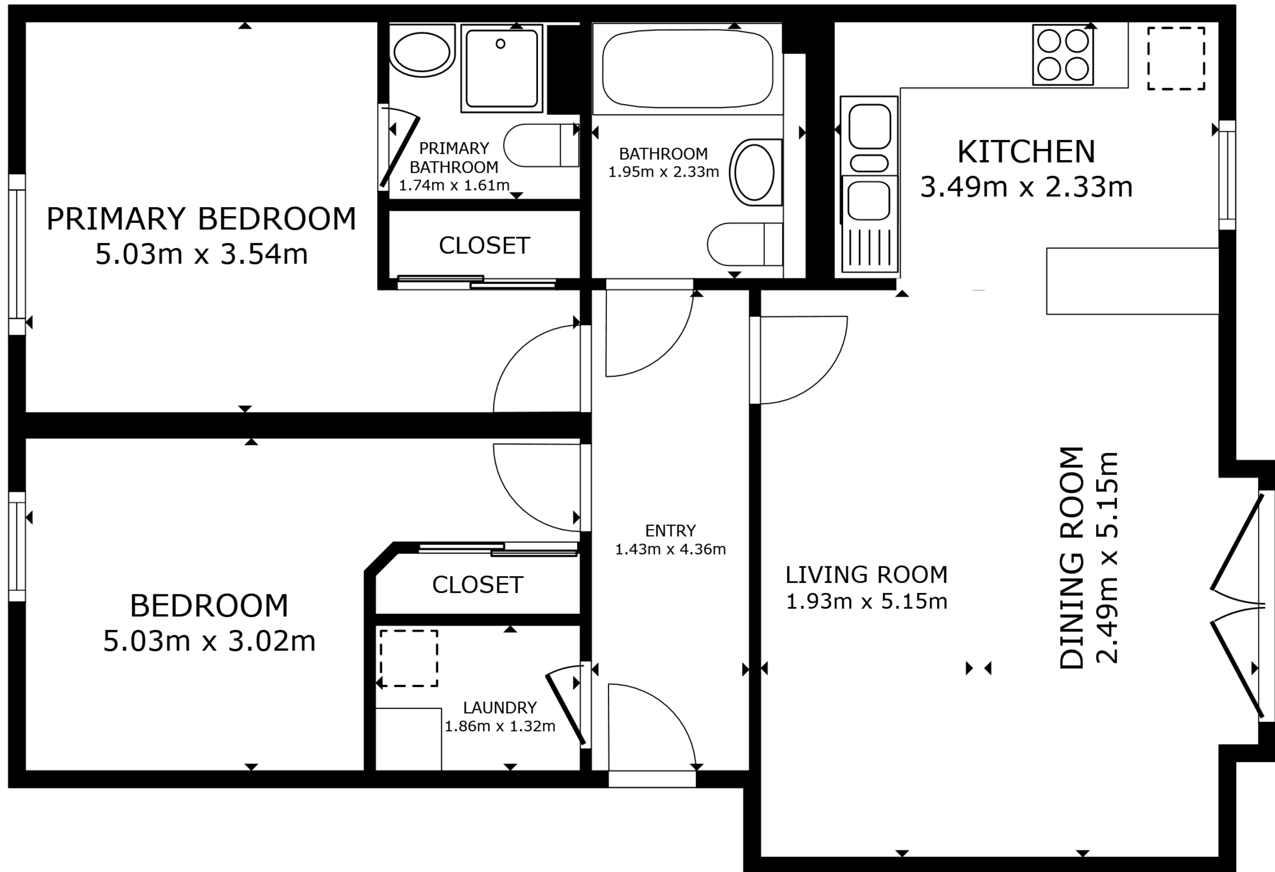
FLOOR PLAN
