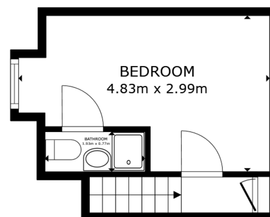
FLOOR PLAN 3
