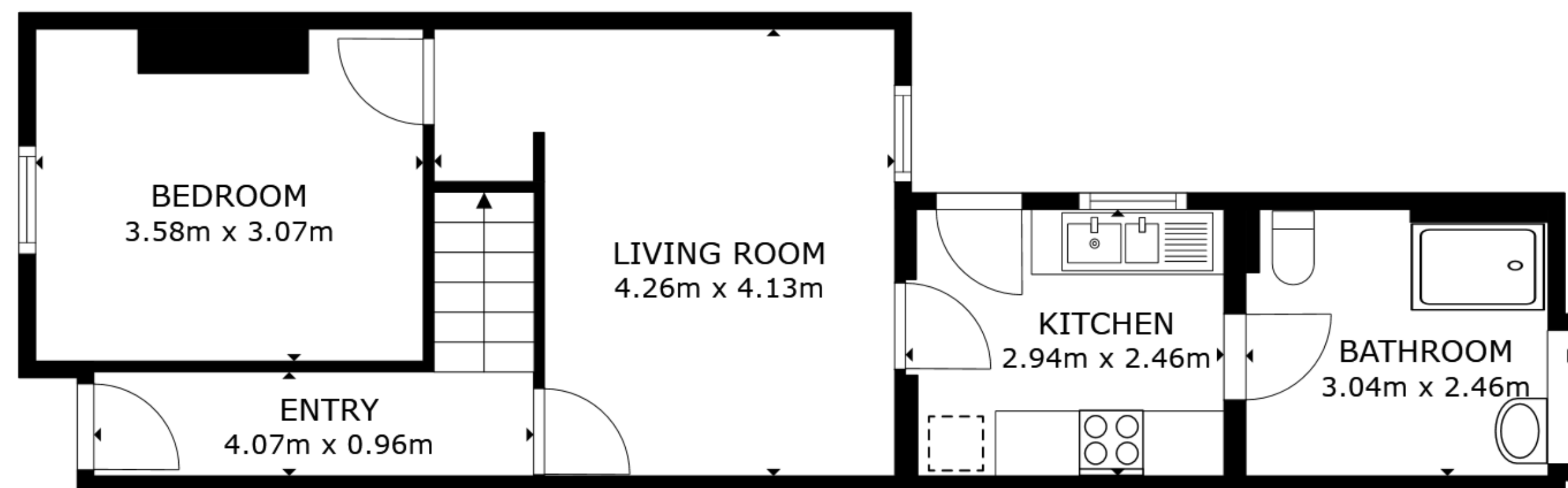
FLOOR 1
