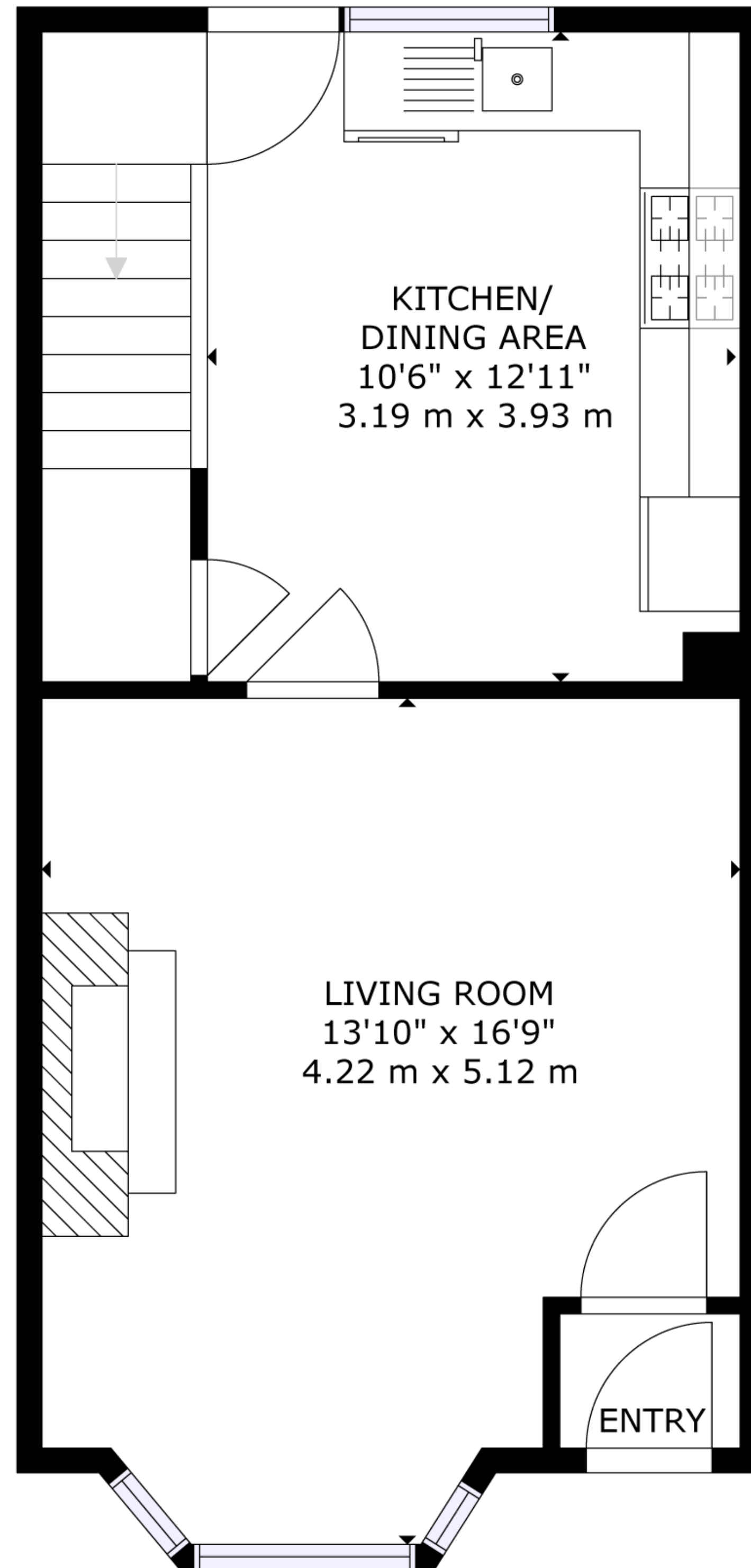
FLOOR 1
