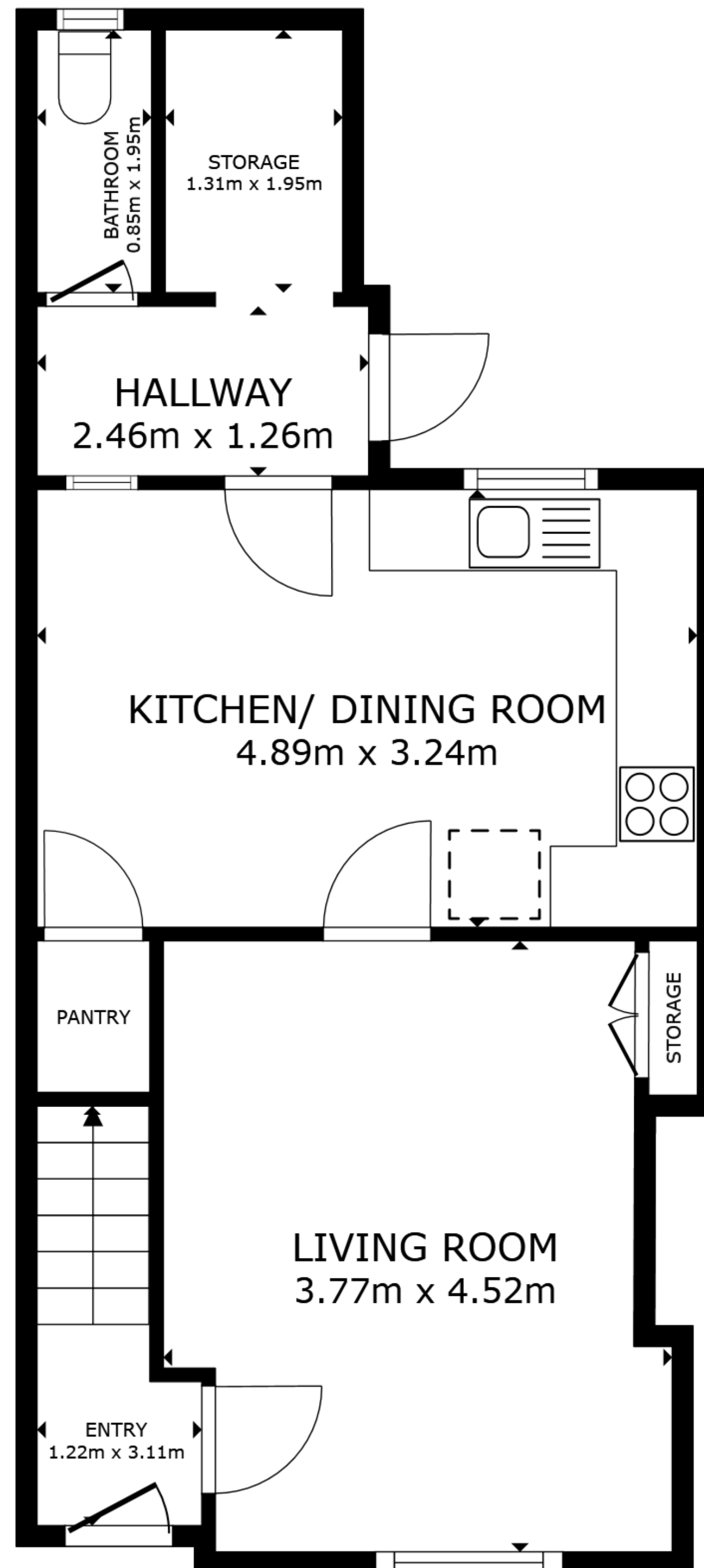
FLOOR 1
