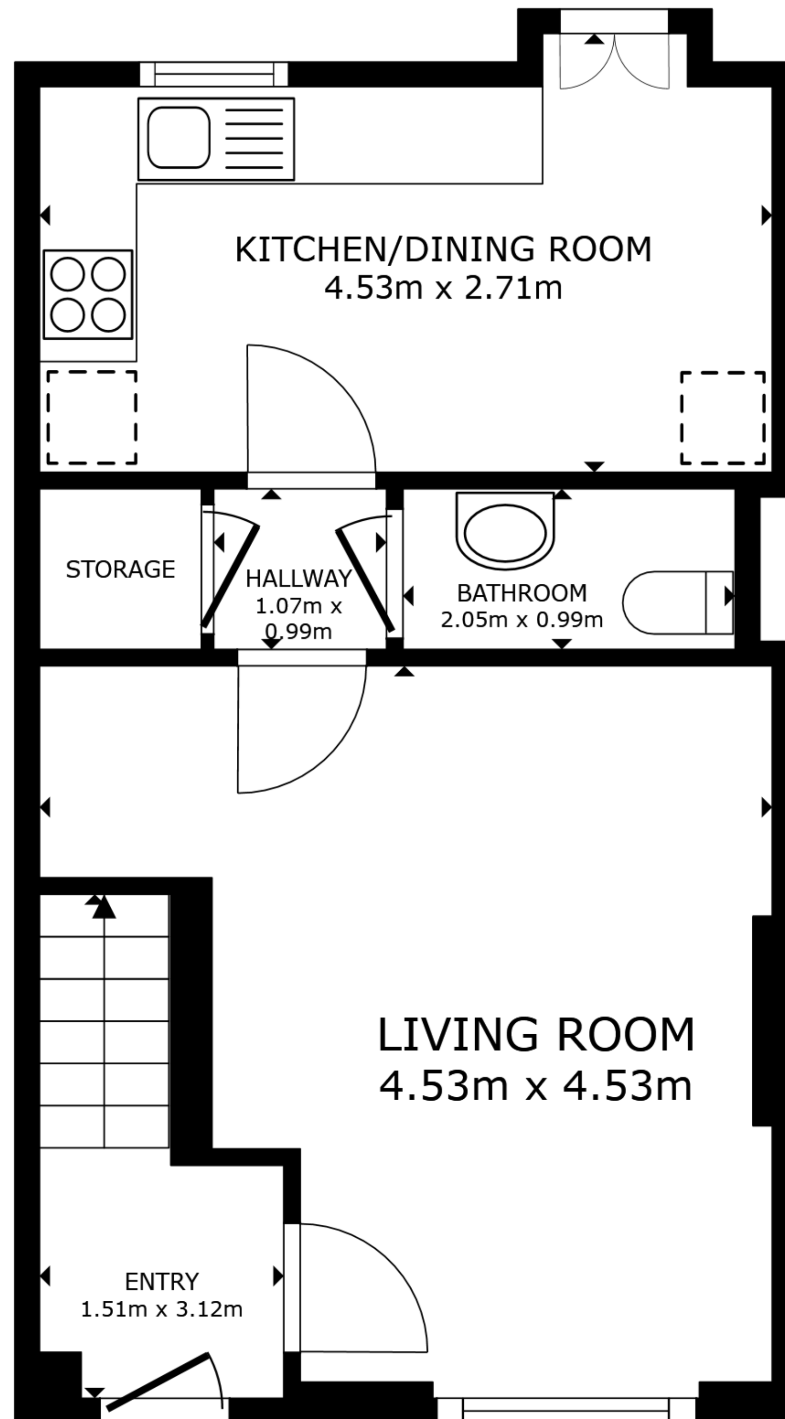
FLOOR 1
