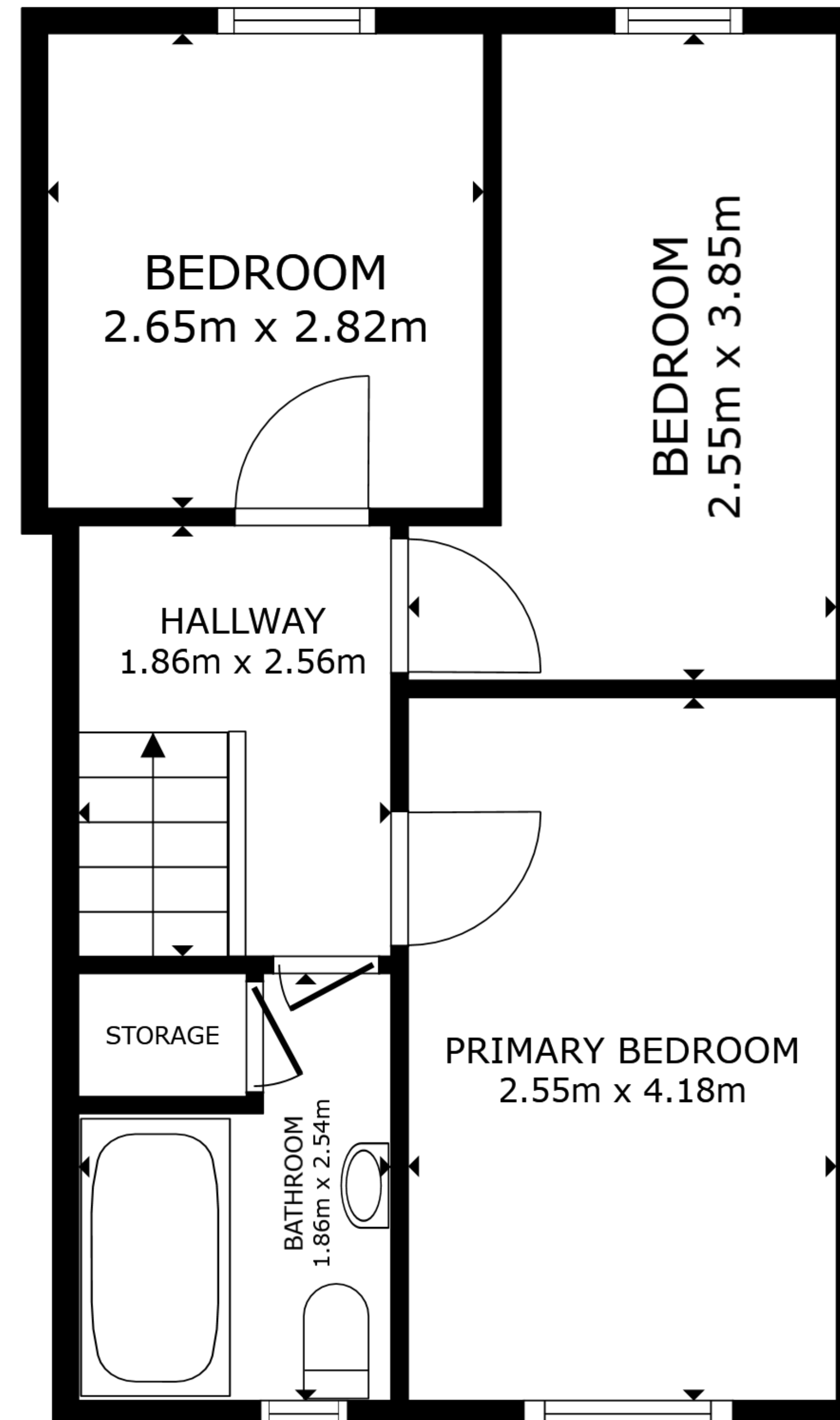
FLOOR 2
