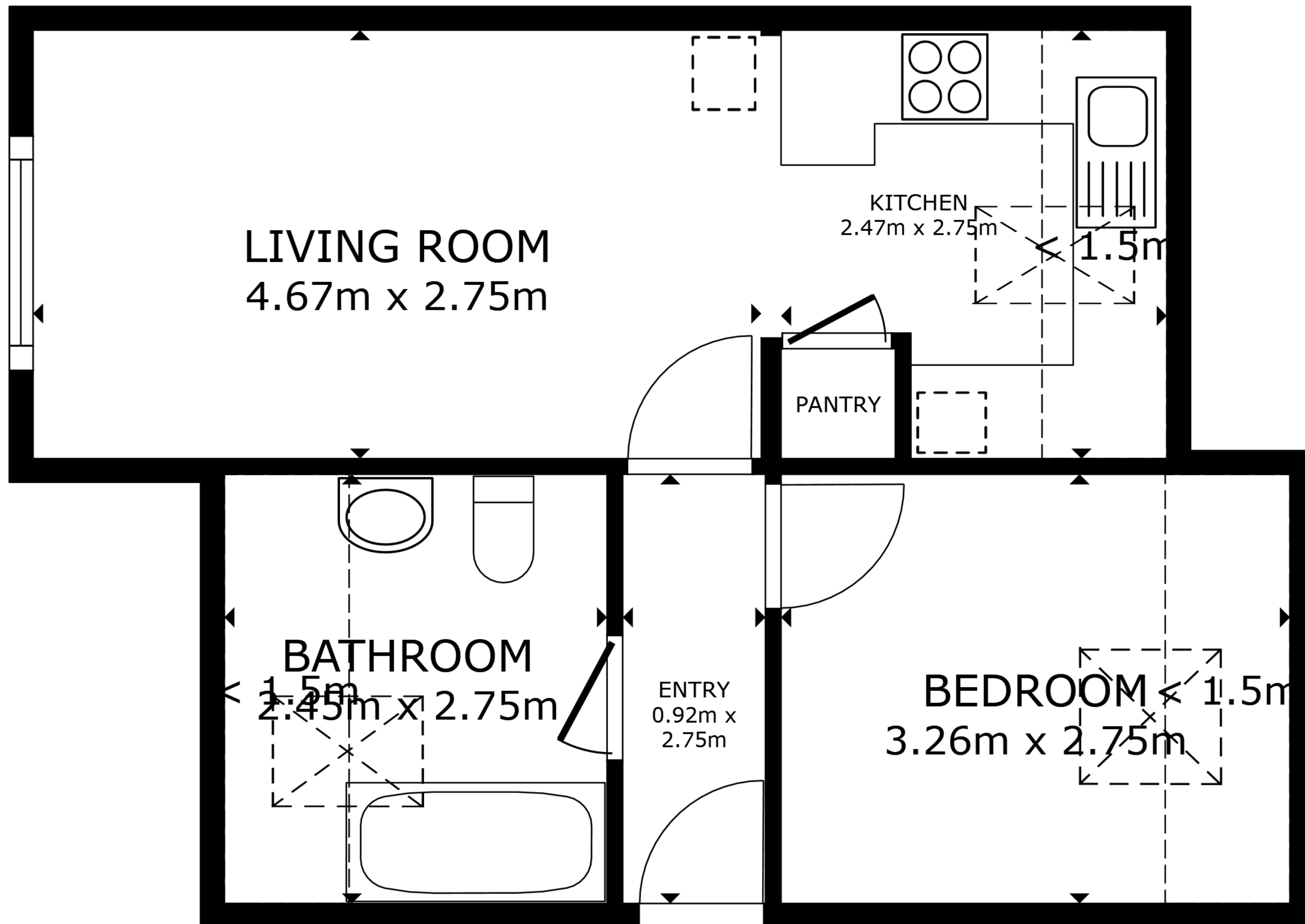
FLOOR PLAN
