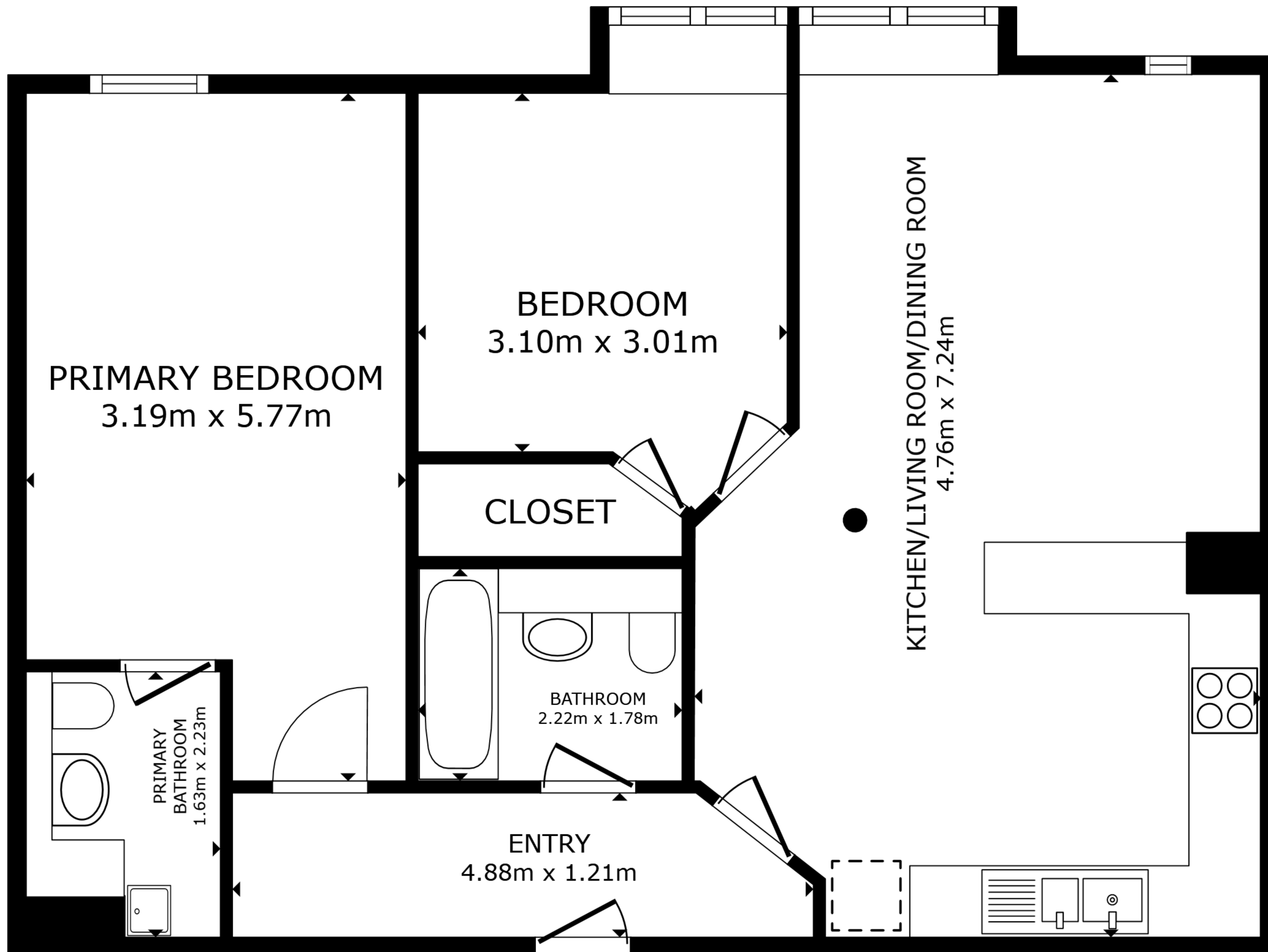
FLOOR PLAN
