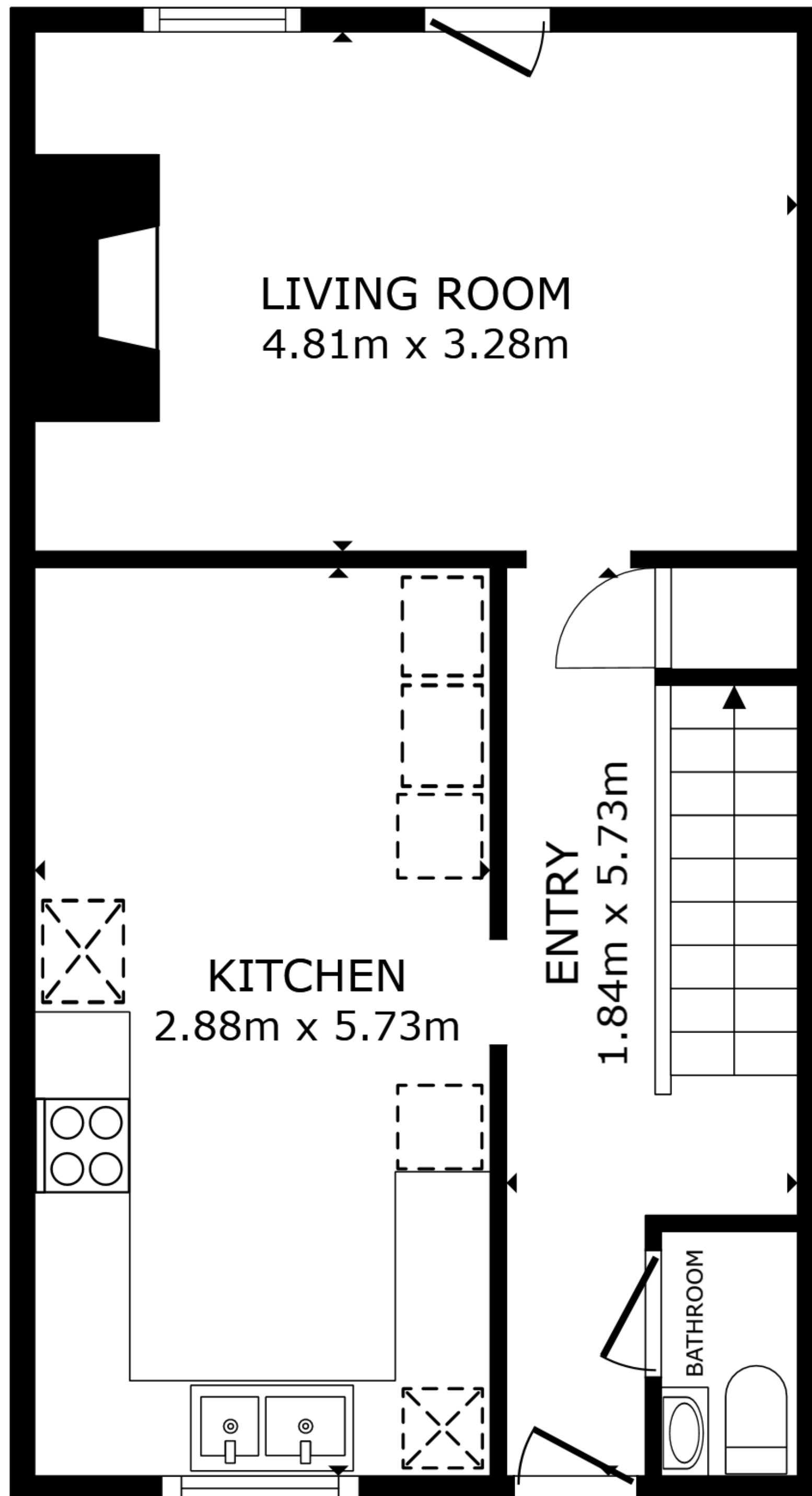
FLOOR 1
