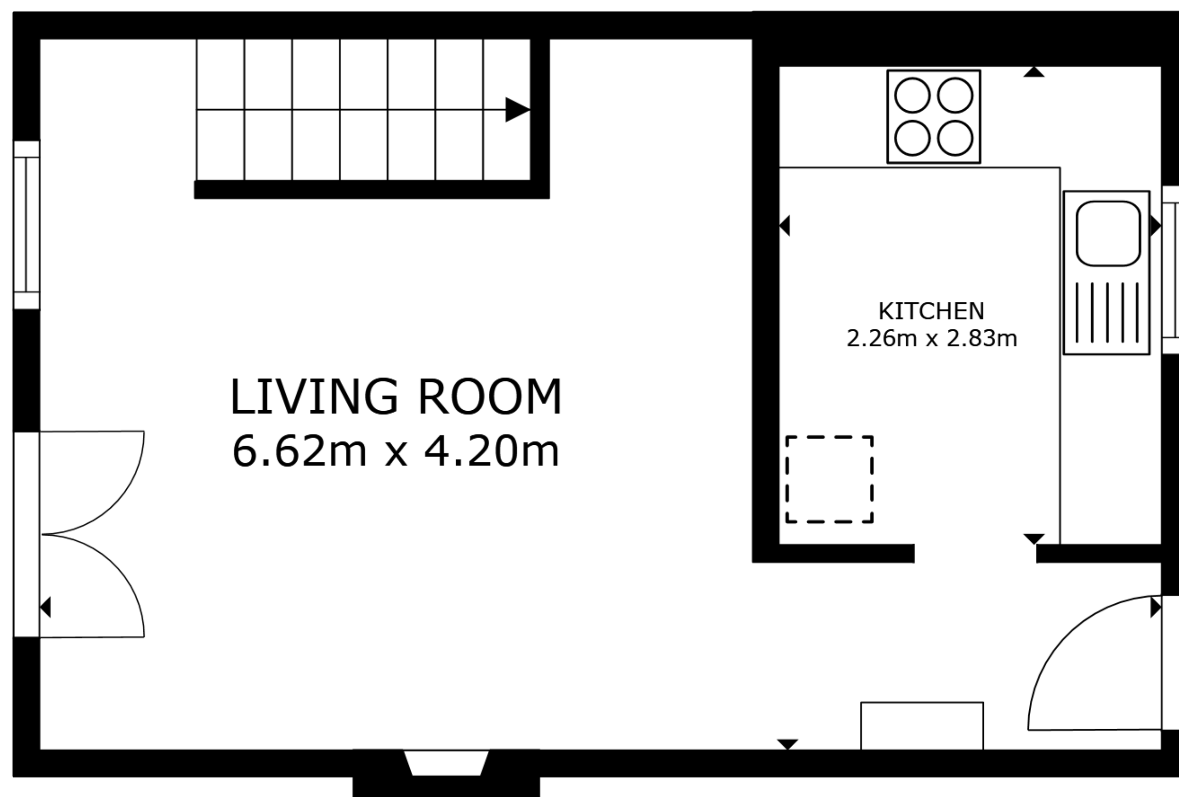
FLOOR 1
